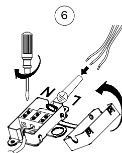
Connect the wires
