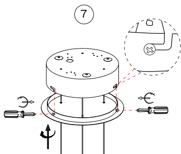
Apply side screws and make Hanging elements stable
