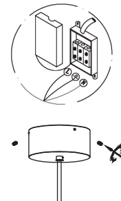
Connect wires
